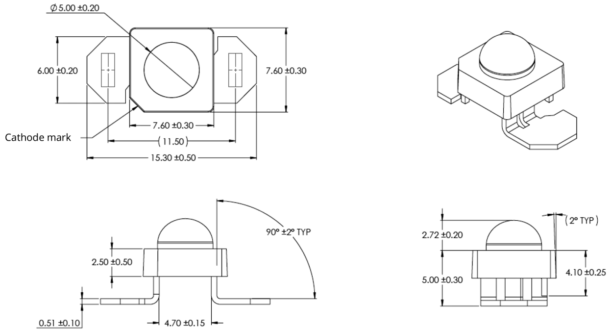
Figure 7b: Mechanical dimensions for SnapLED 150 wide lens.
