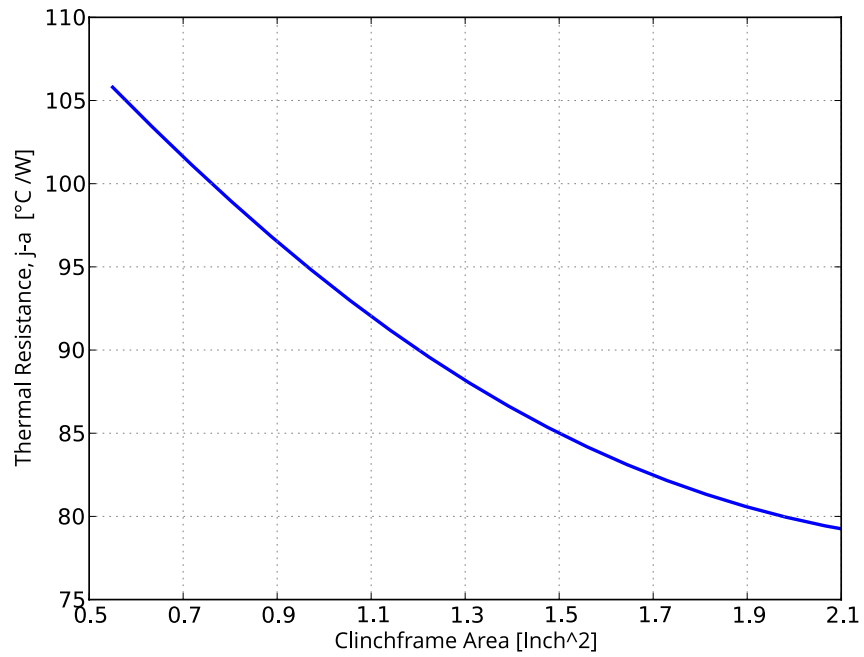
Figure 8: Approximate total thermal resistance vs. clinch frame area per anode for SnapLED 150.
