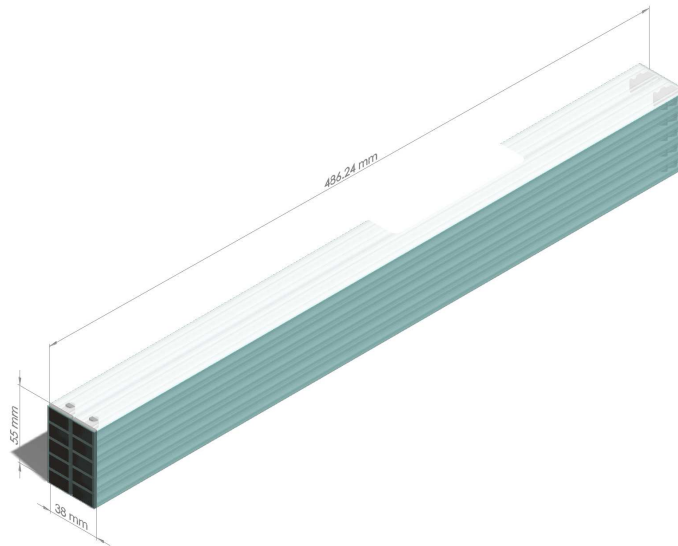
Figure 11a: Bundle dimensions for SnapLED 150.
