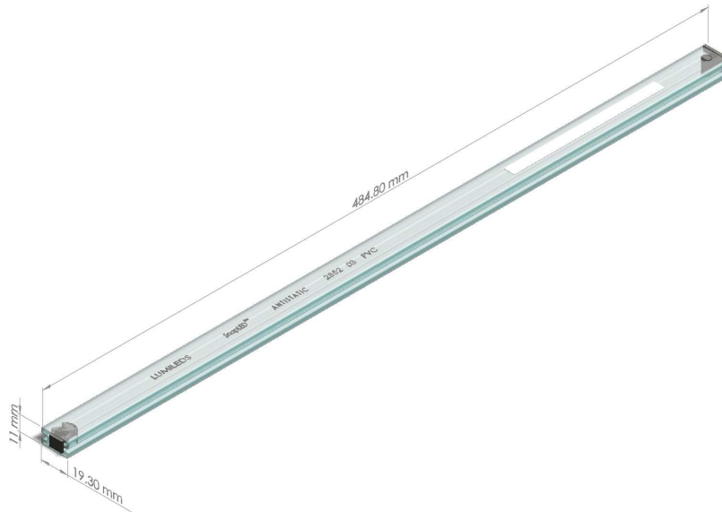
Figure 9: Tube dimensions for SnapLED 150.
