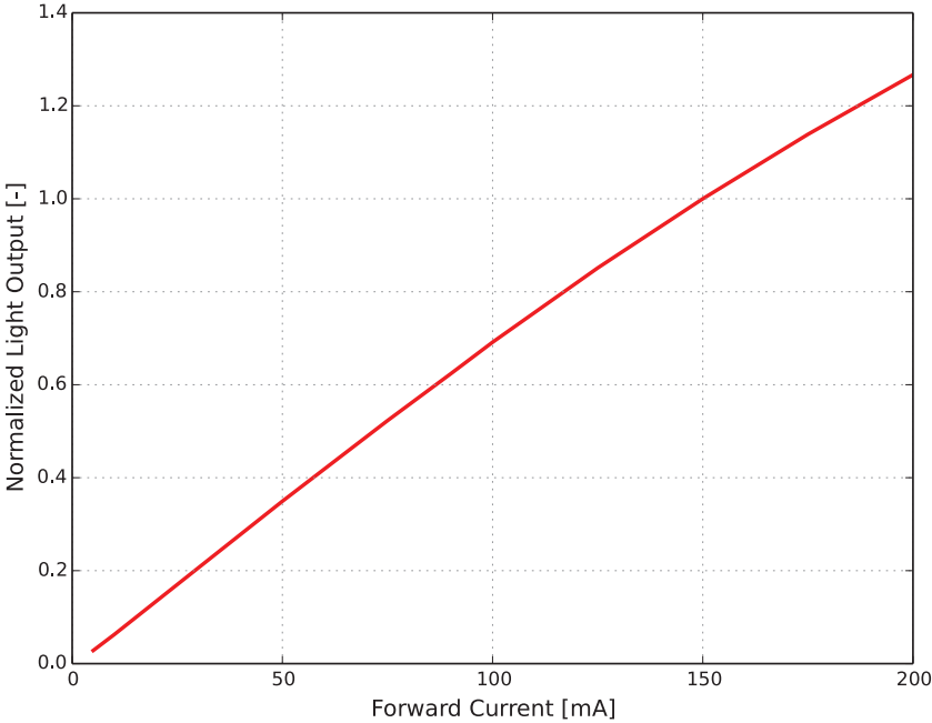
Figure 3: Typical normalized light output vs. forward current for SnapLED 150 at T_j=25^\circ\text{C} .
