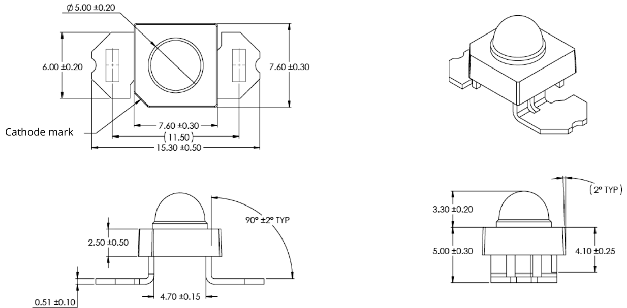
Figure 7a: Mechanical dimensions for SnapLED 150 narrow lens.
