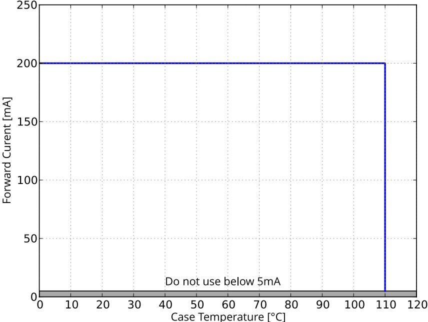
Figure 6: Maximum forward current vs. case temperature for SnapLED 150.
